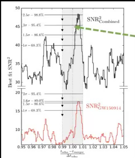
FIG. 4: Best fit (or maximum) \text{SNR}^2 near the expected time of merger echoes (Eq's. 1 and 6), for the combined (top) and GW150914 (bottom) events. The significance of the peaks is quantified by the p-value of their \text{SNR}_{\text{max}} within the gray rectangle (see Appendix E for detail of calculation).
