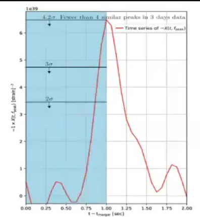
FIG. 6: Amplitude-time representations of first (and most significant) echo peak at 1.0 sec after the merger and frequency of 72 Hz. The shaded region is 0-1 sec: prior range after the merger, first adopted in [21], which we use to estimate p-value. The maximum of the peak is 6.48 \times 10^{39} .
