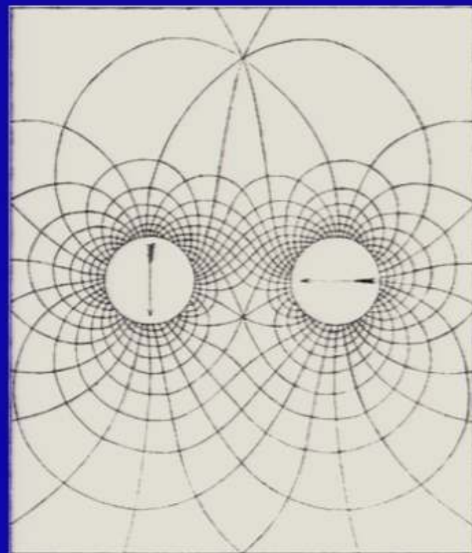
Two Cylinders magnetized transversely.
